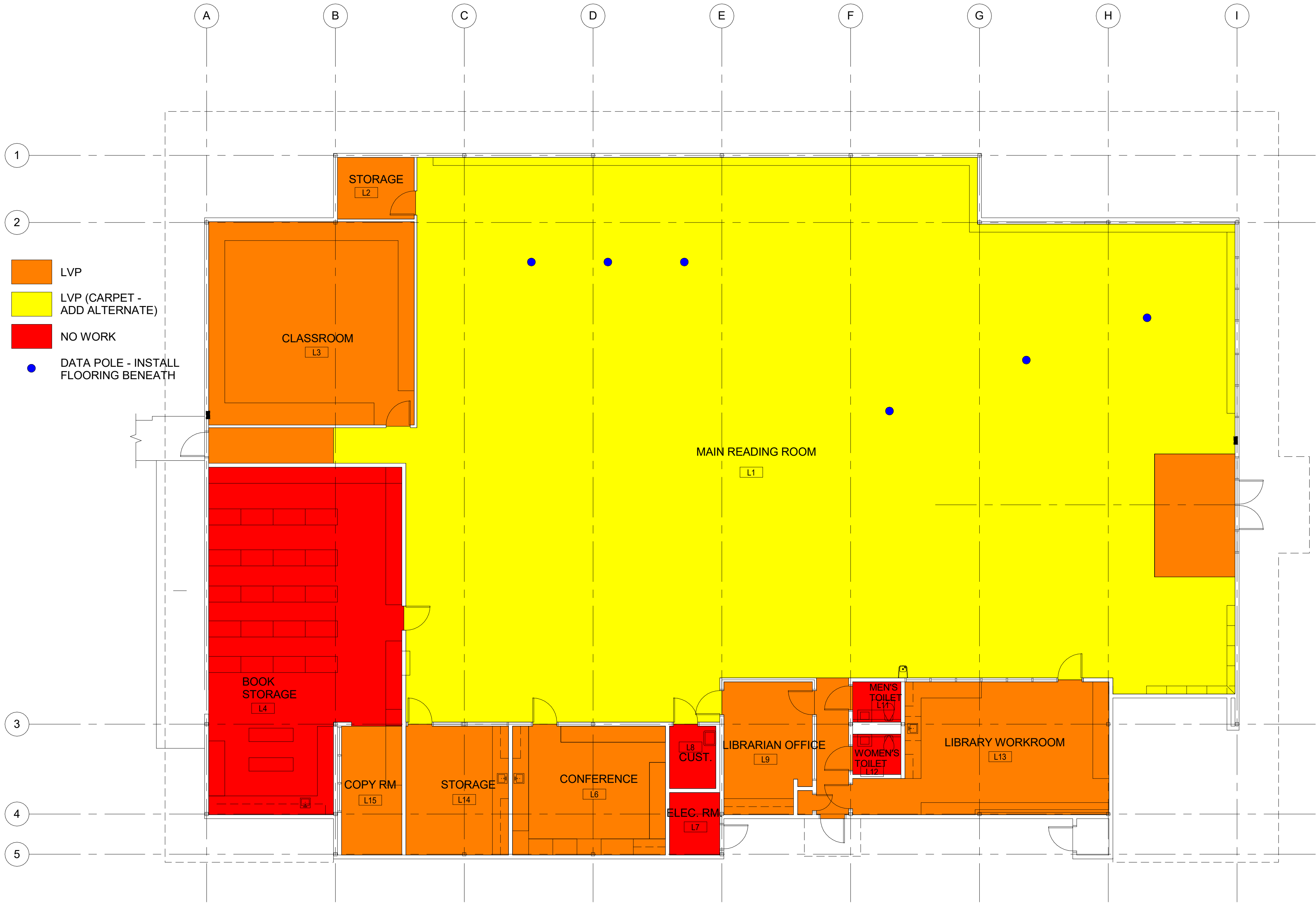
1 EDISON HIGH SCHOOL LIBRARY FLOOR FINISHES PLAN 1/8" = 1'-0"
